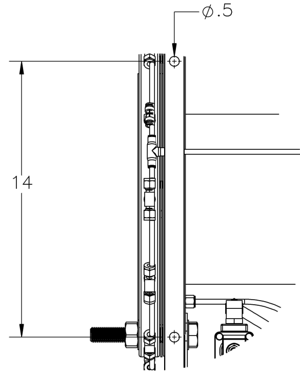
DETAIL A
